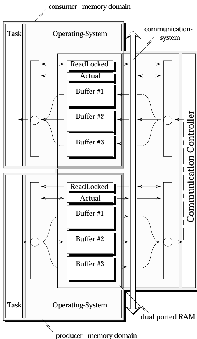
figure 5: the communication-controller
