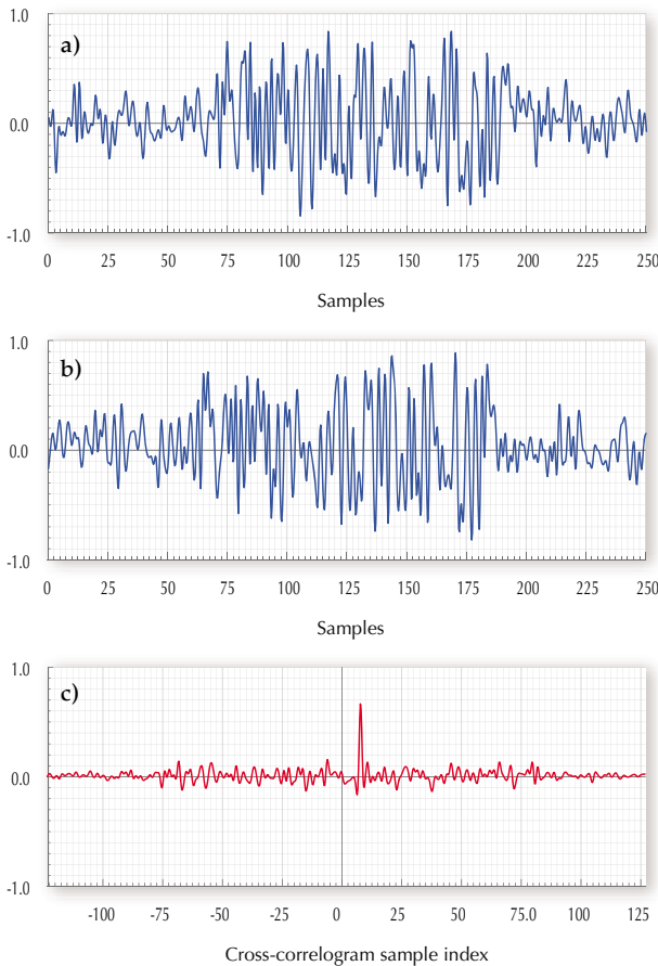
Figure 1: Plot shown in c) results from the cross-correlation of the shifted noisy MLS signals shown in a) and b). In each plot, the y-axis reprinter normalised amplitude.
