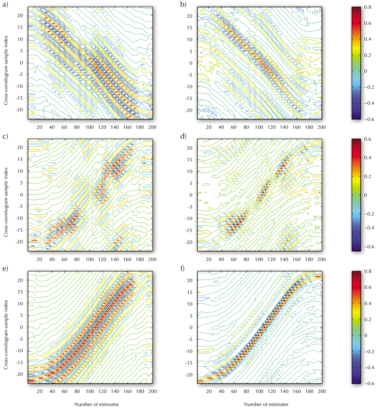
Figure 6: Contour plots shows series of cross-correlograms resulting from three different experiments shown on three rows.
