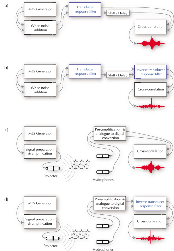
Figure 3: The four different setups producing the four different cross-correlograms shown in Figure 4.
